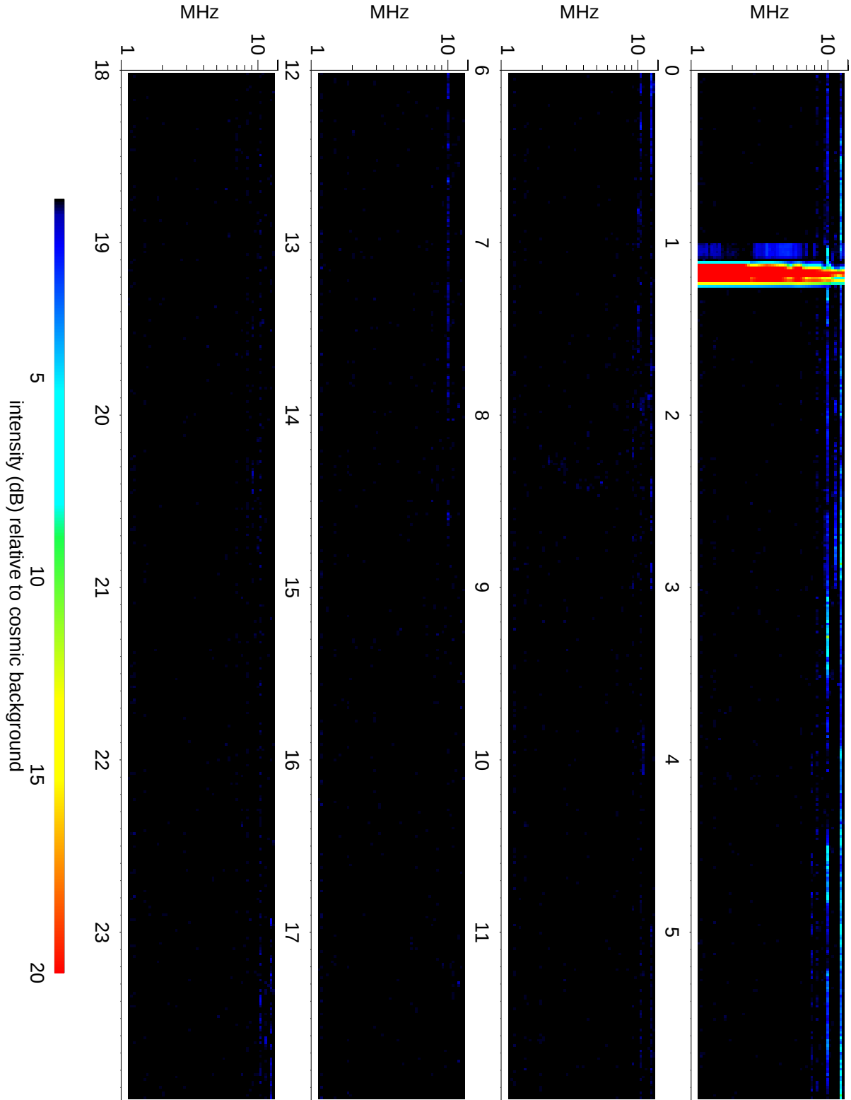
Wind Waves RAD2 receiver: 2019/11/06
