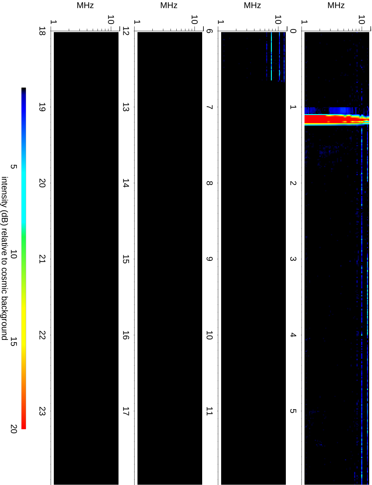
Wind Waves RAD2 receiver: 2019/06/03
