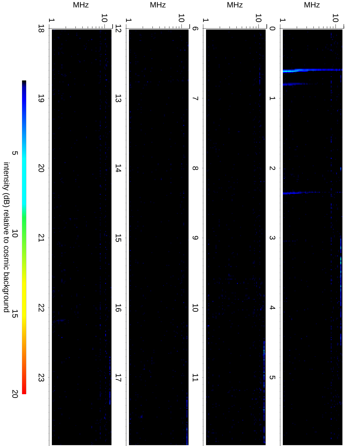
Wind Waves RAD2 receiver: 2015/11/15
