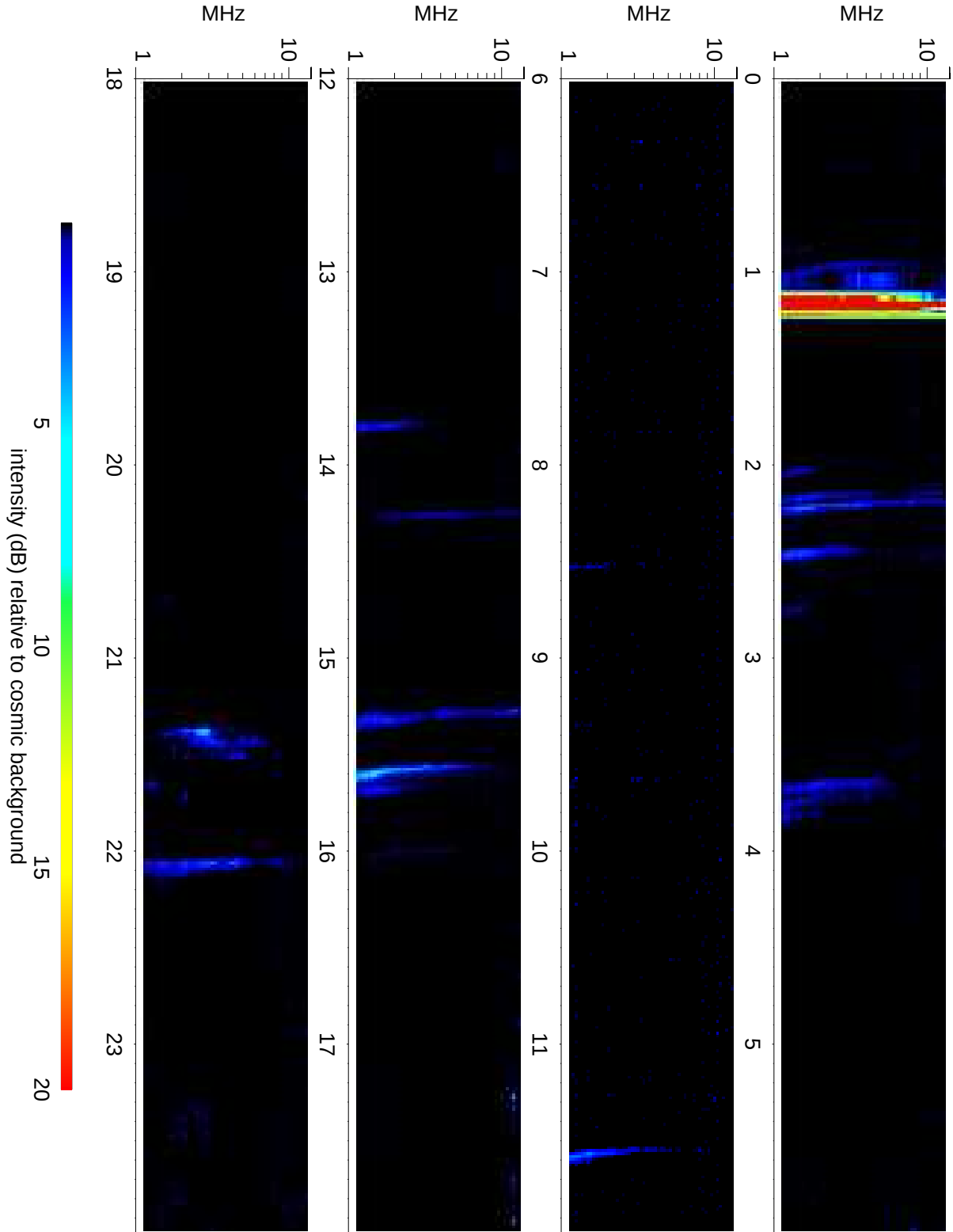
Wind Waves RAD2 receiver: 2014/01/16
