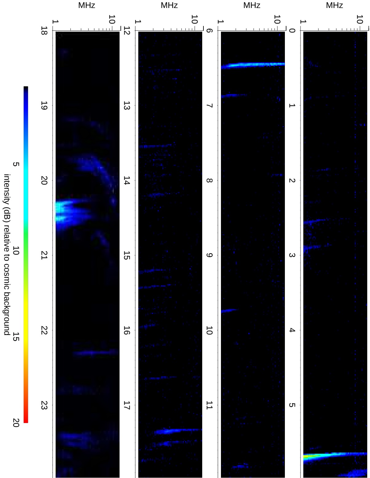
Wind Waves RAD2 receiver: 2011/12/23
