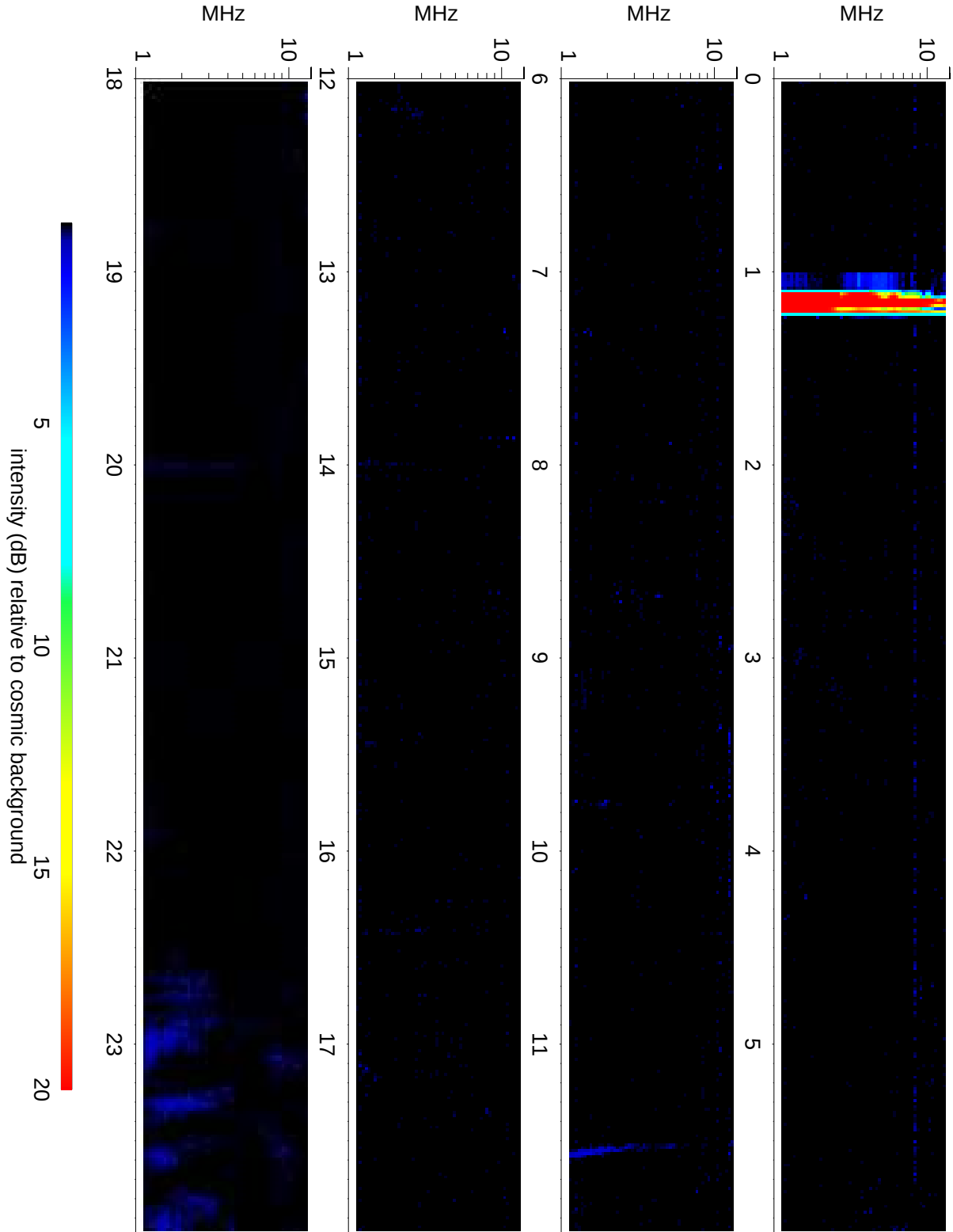
Wind Waves RAD2 receiver: 2011/12/16
