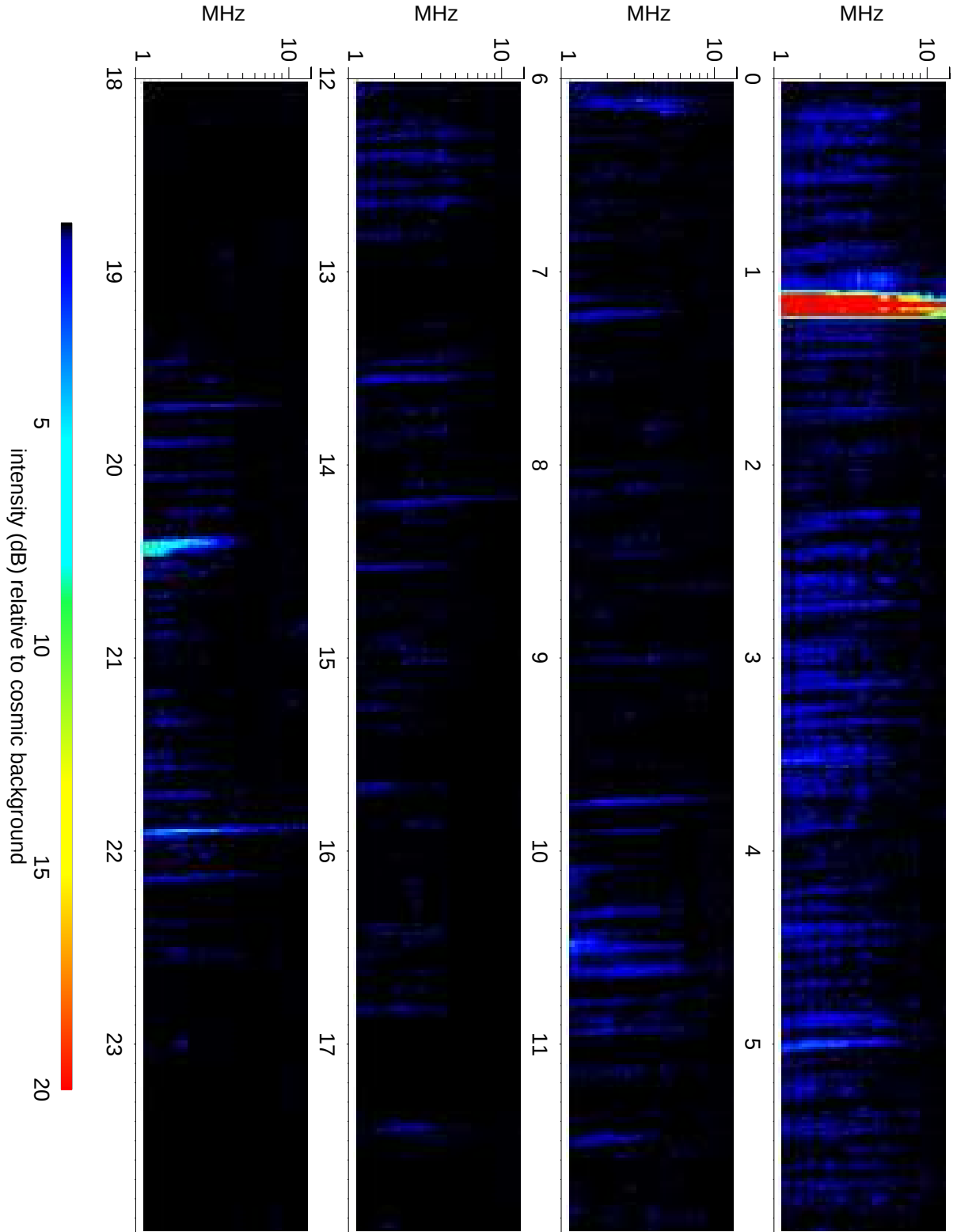
Wind Waves RAD2 receiver: 2011/11/20/06
