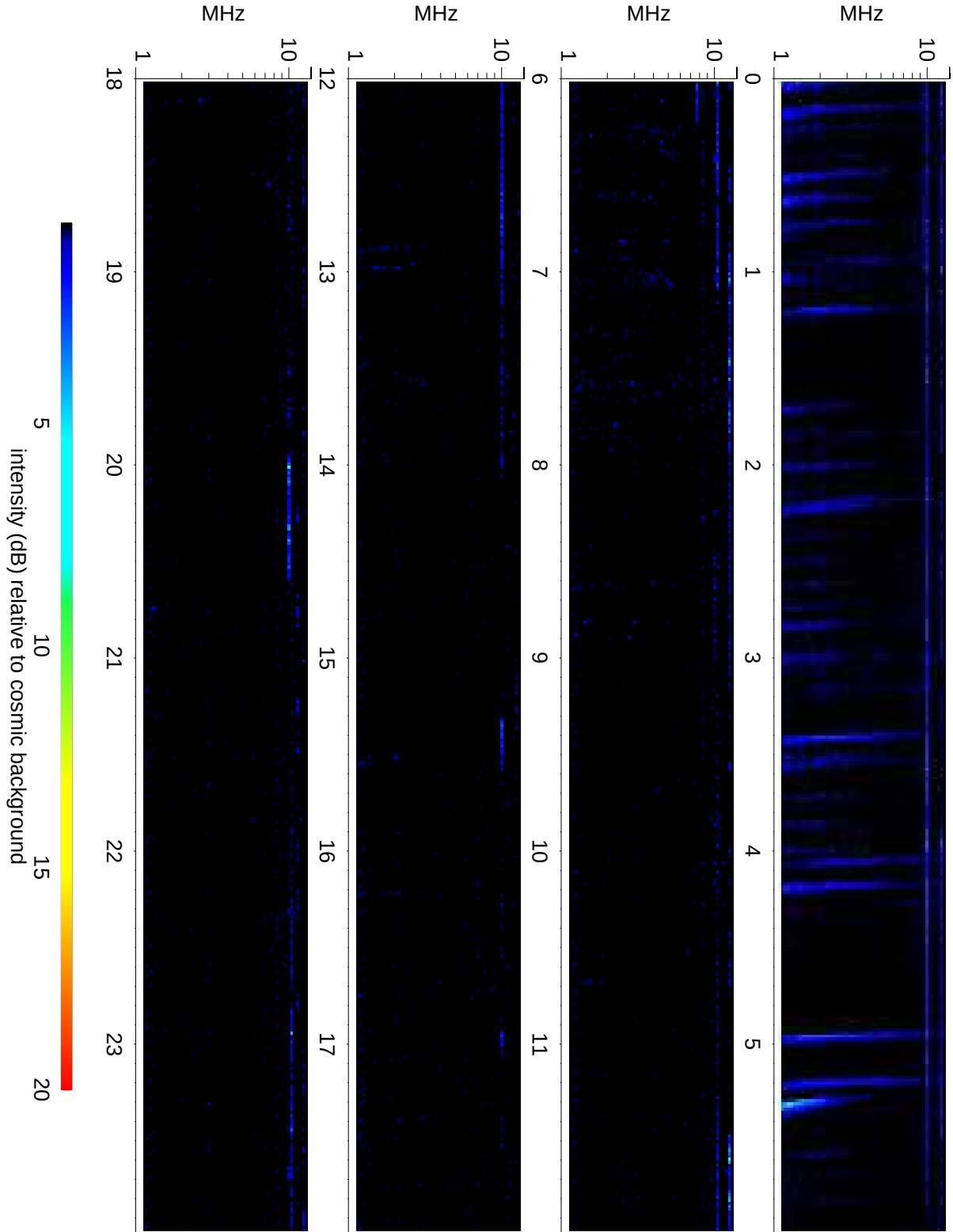
Wind Waves RAD2 receiver: 2011/06/20
