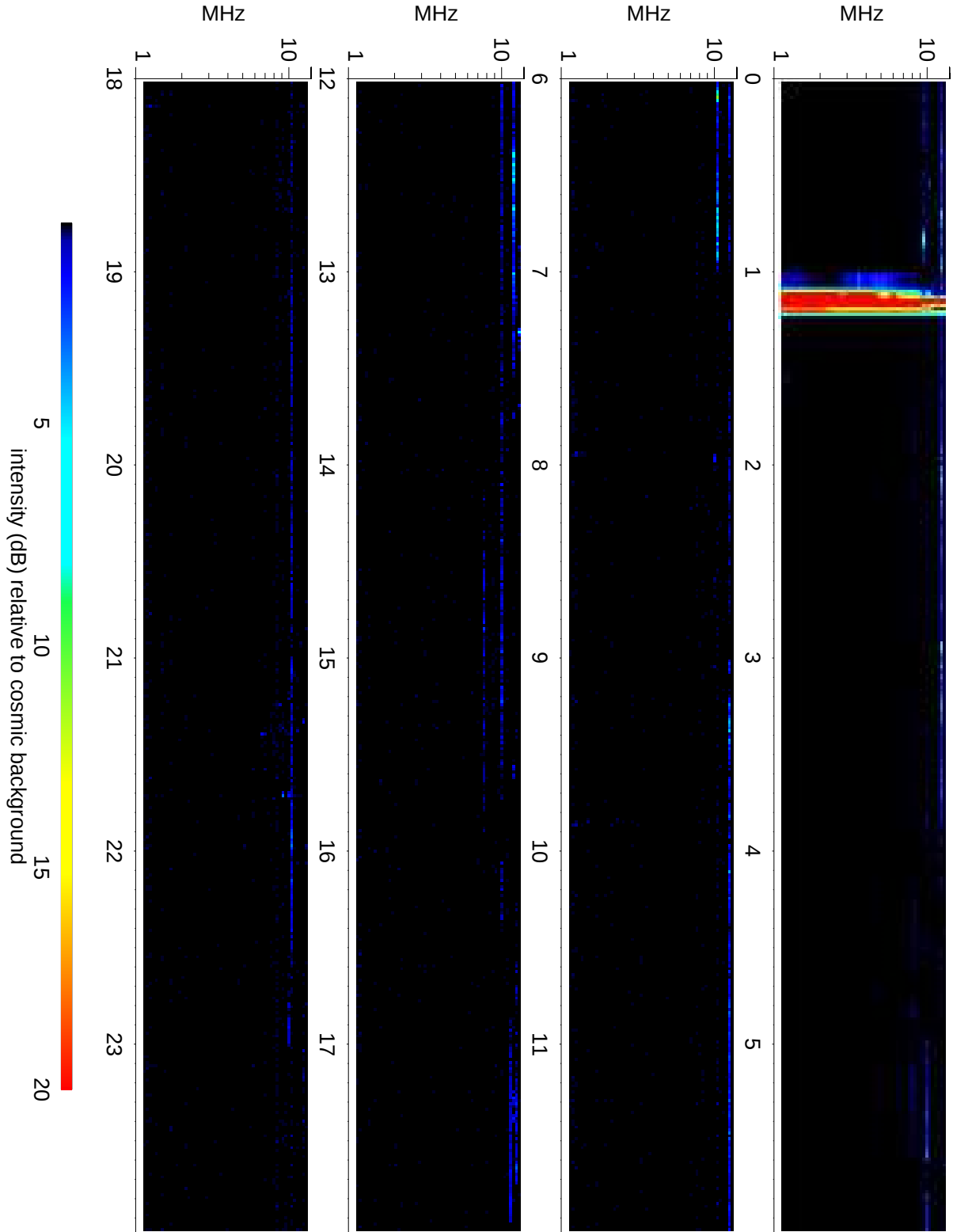
Wind Waves RAD2 receiver: 2011/01/06
