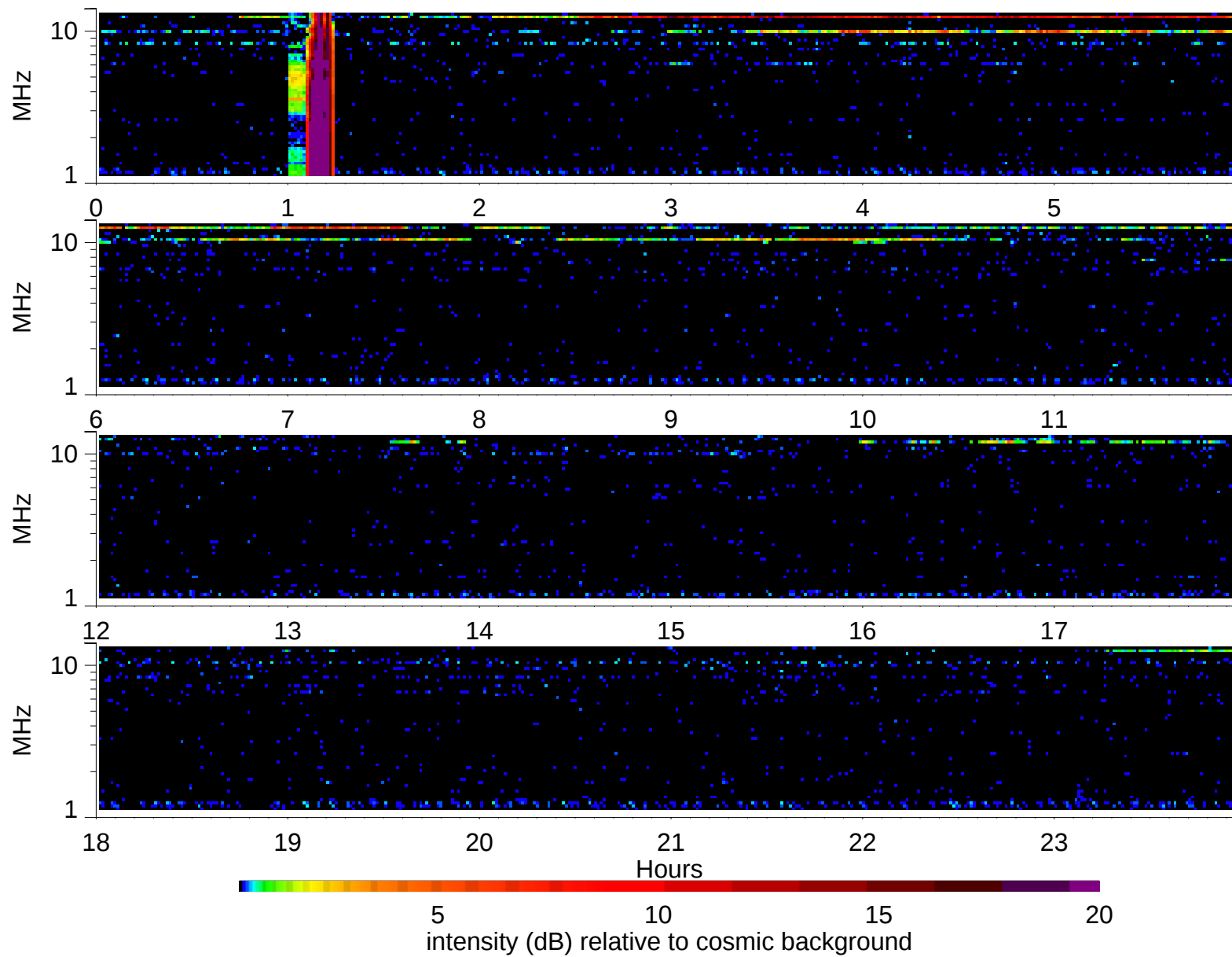
Wind Waves RAD2 receiver: 2007/12/20
