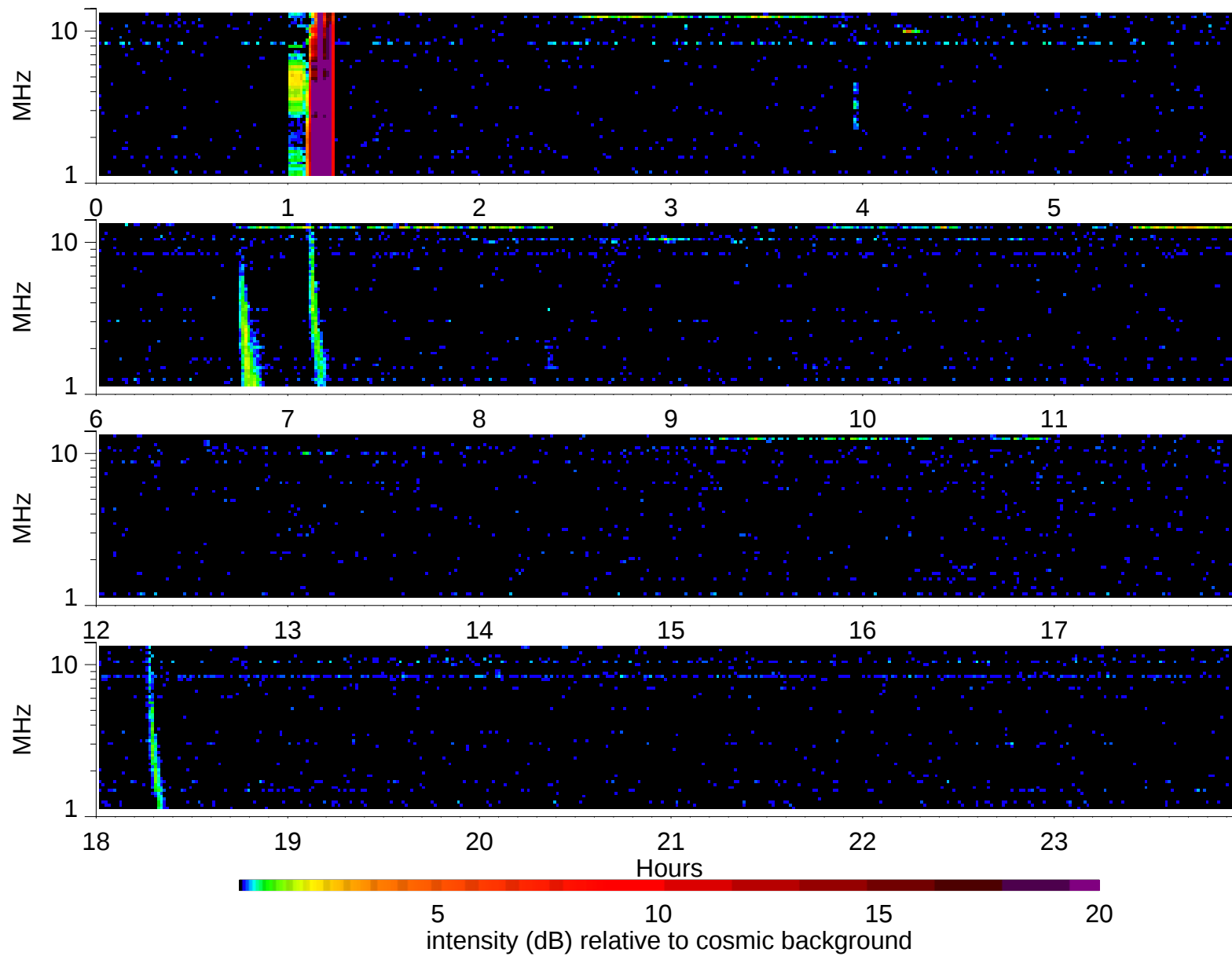
Wind Waves RAD2 receiver: 2005/10/13
