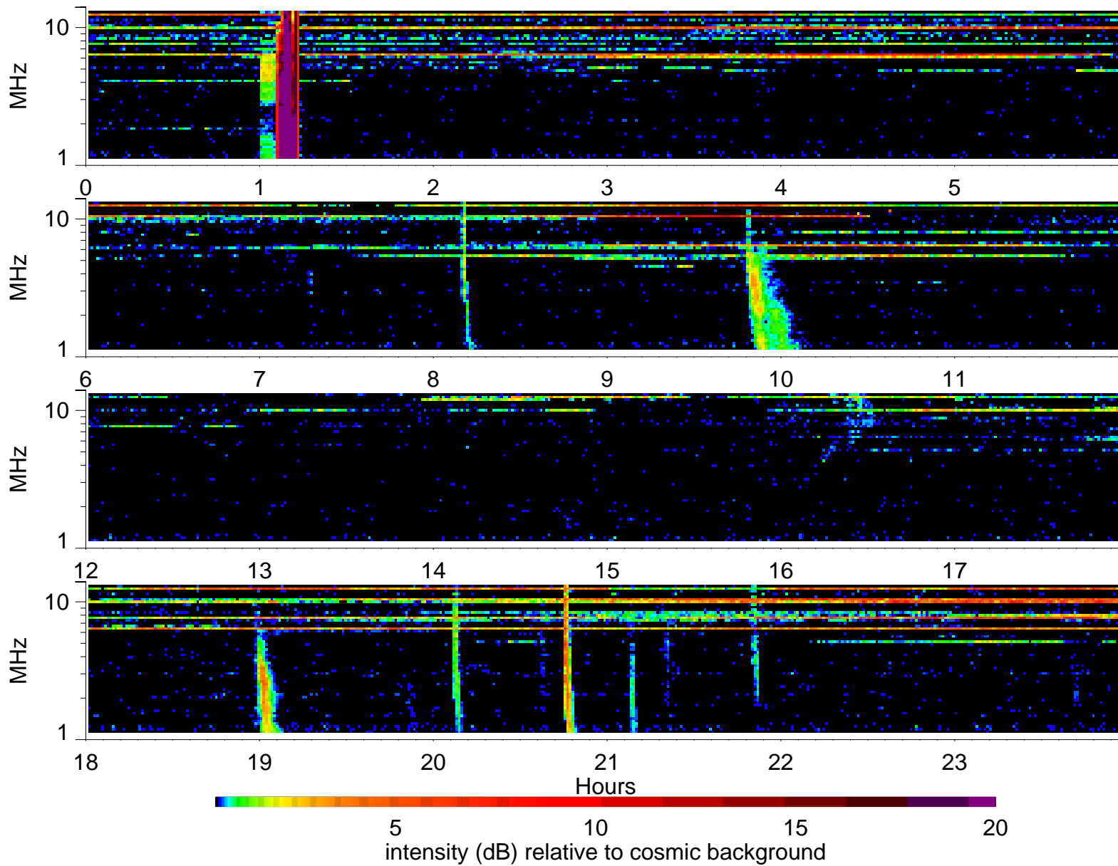
Wind Waves RAD2 receiver: 2003/9/3
