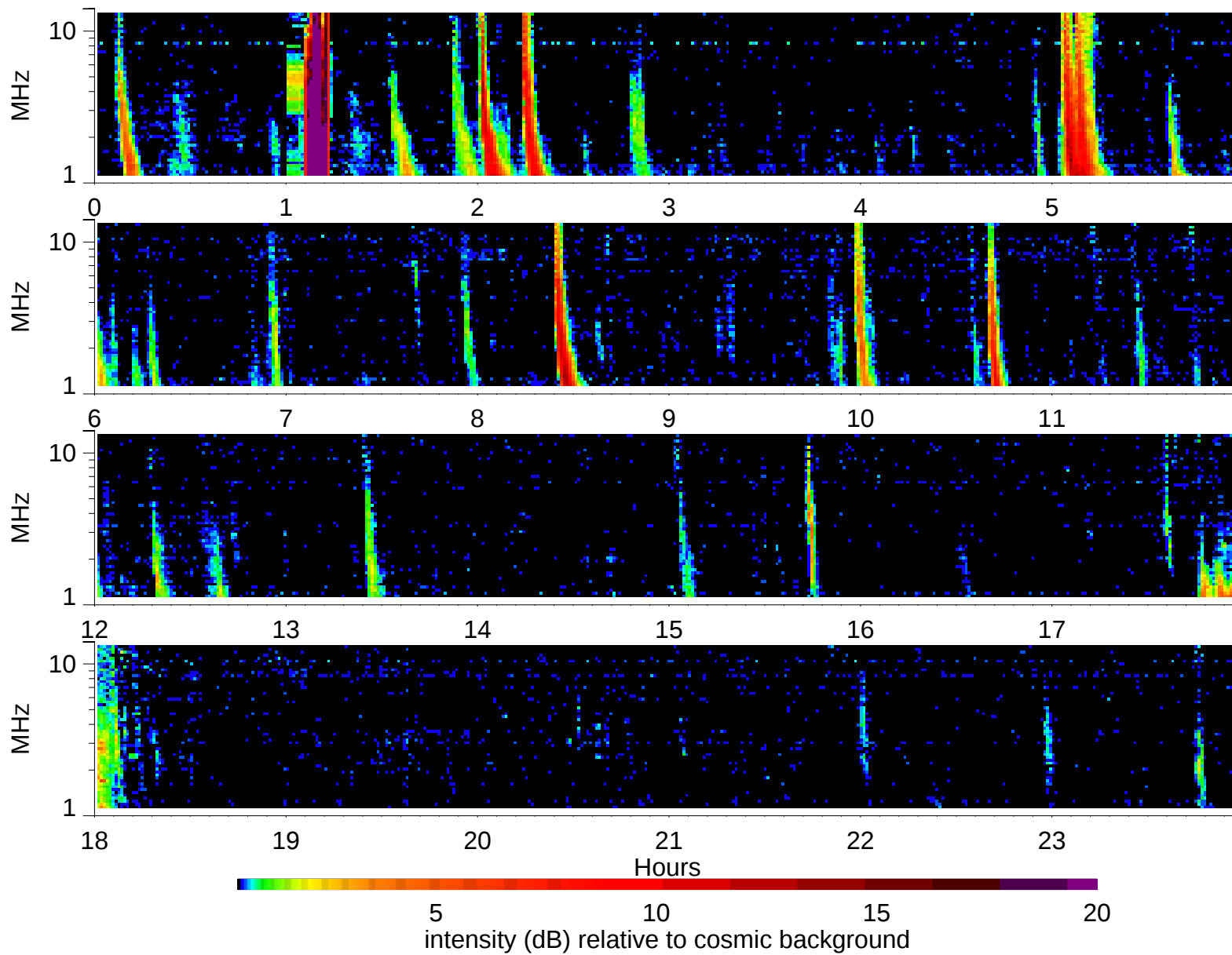
Wind Waves RAD2 receiver: 2002/11/8
