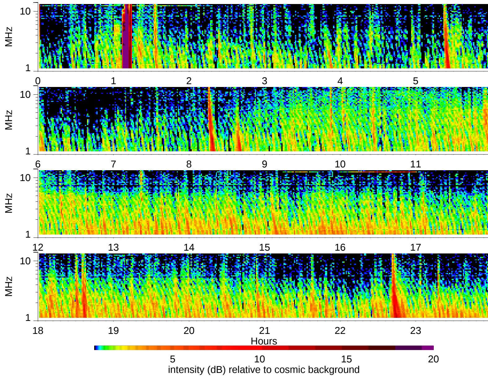
Wind Waves RAD2 receiver: 2002/9/19
