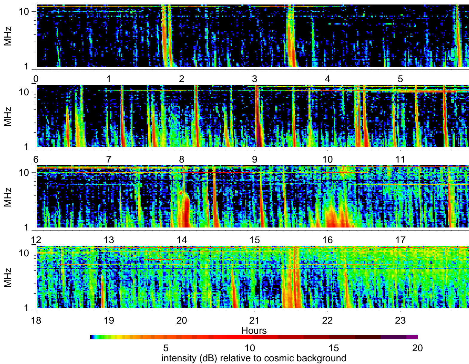
Wind Waves RAD2 receiver: 2002/7/16
