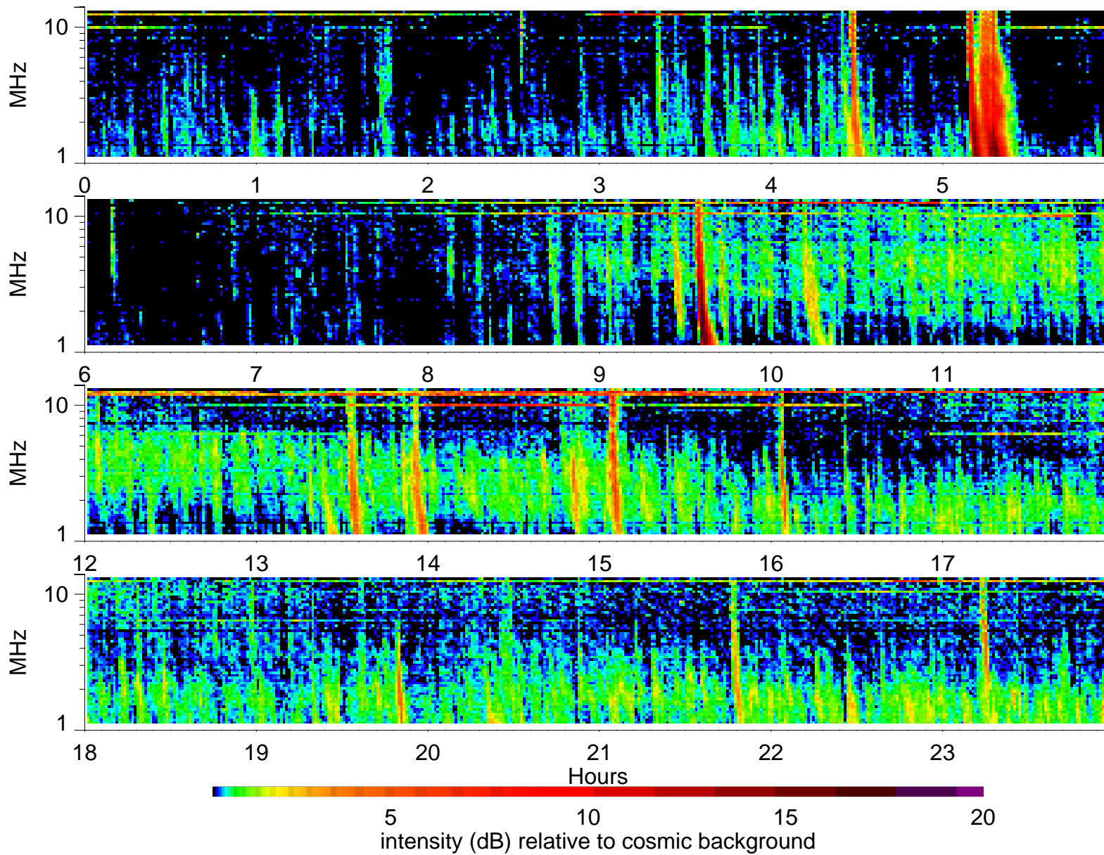
Wind Waves RAD2 receiver: 2002/7/14
