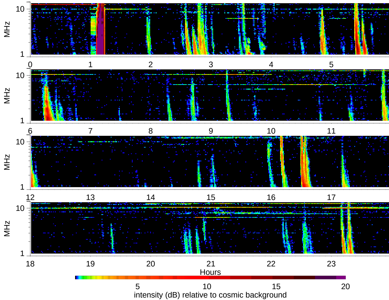
Wind Waves RAD2 receiver: 2002/2/27
