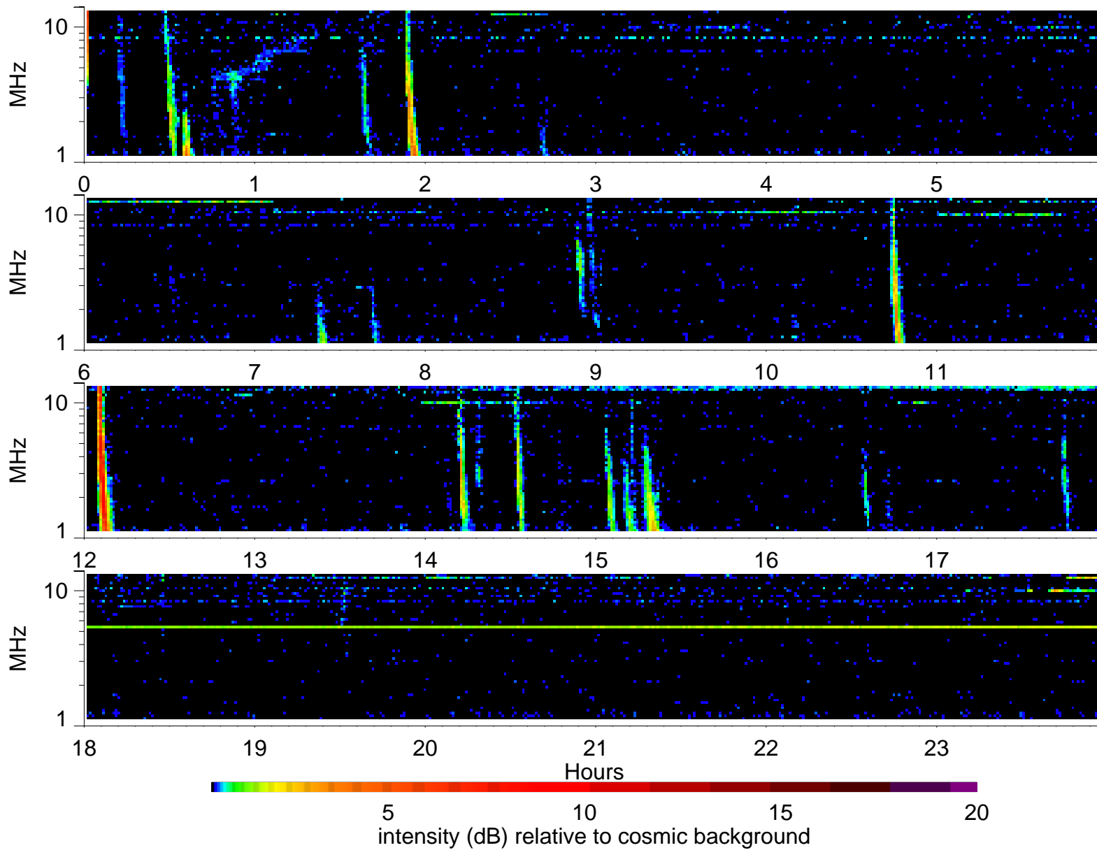
Wind Waves RAD2 receiver: 2001/8/17
