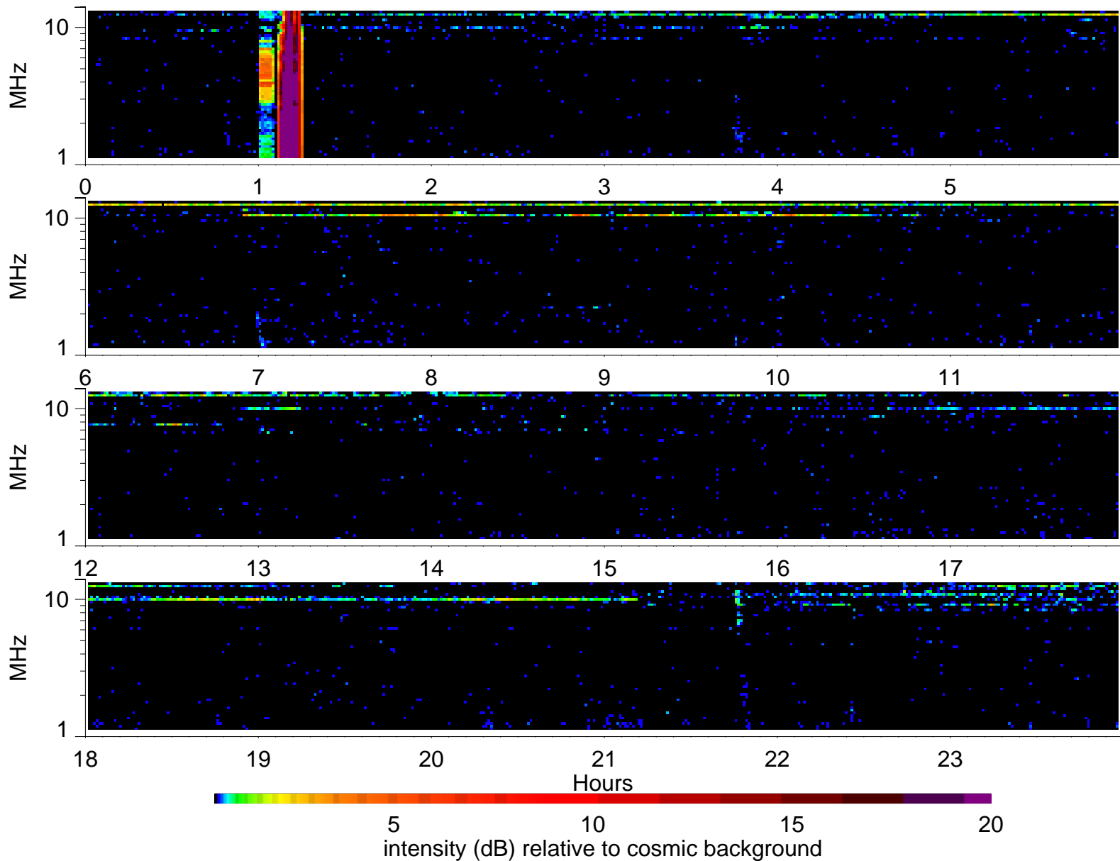
Wind Waves RAD2 receiver: 1998/4/22
