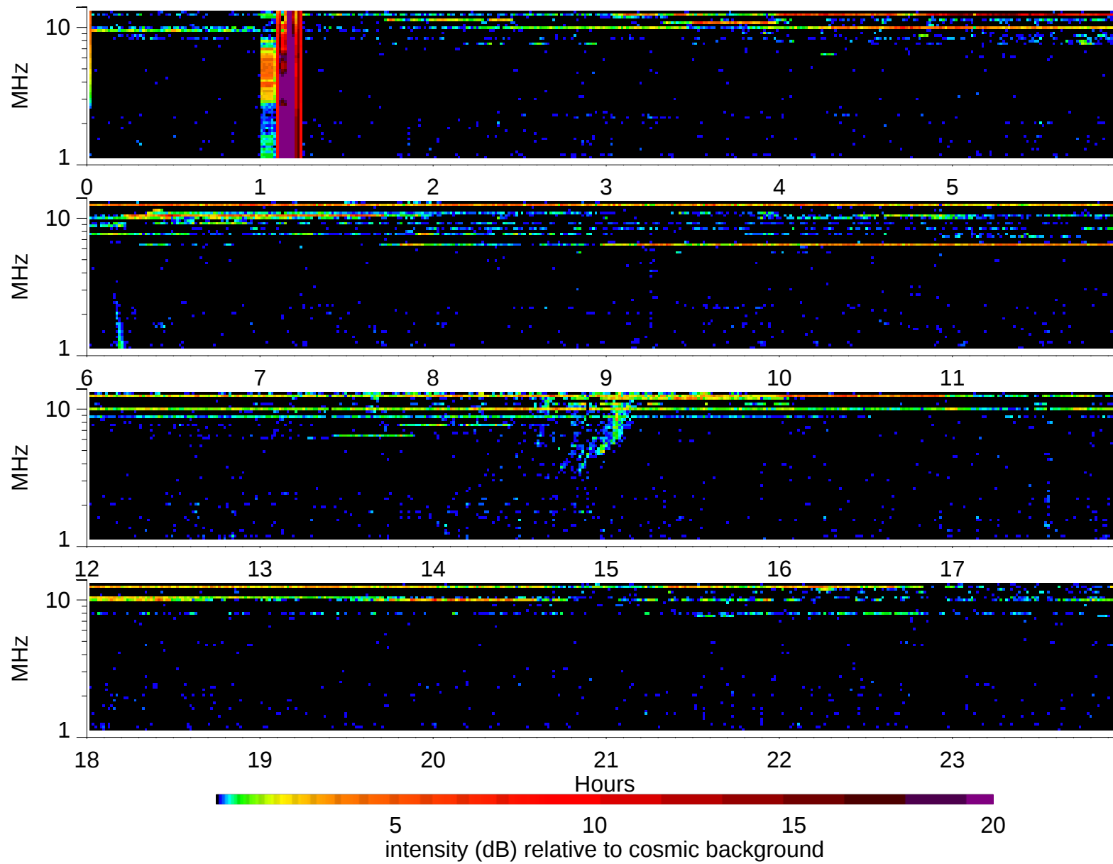
Wind Waves RAD2 receiver: 1997/5/18
