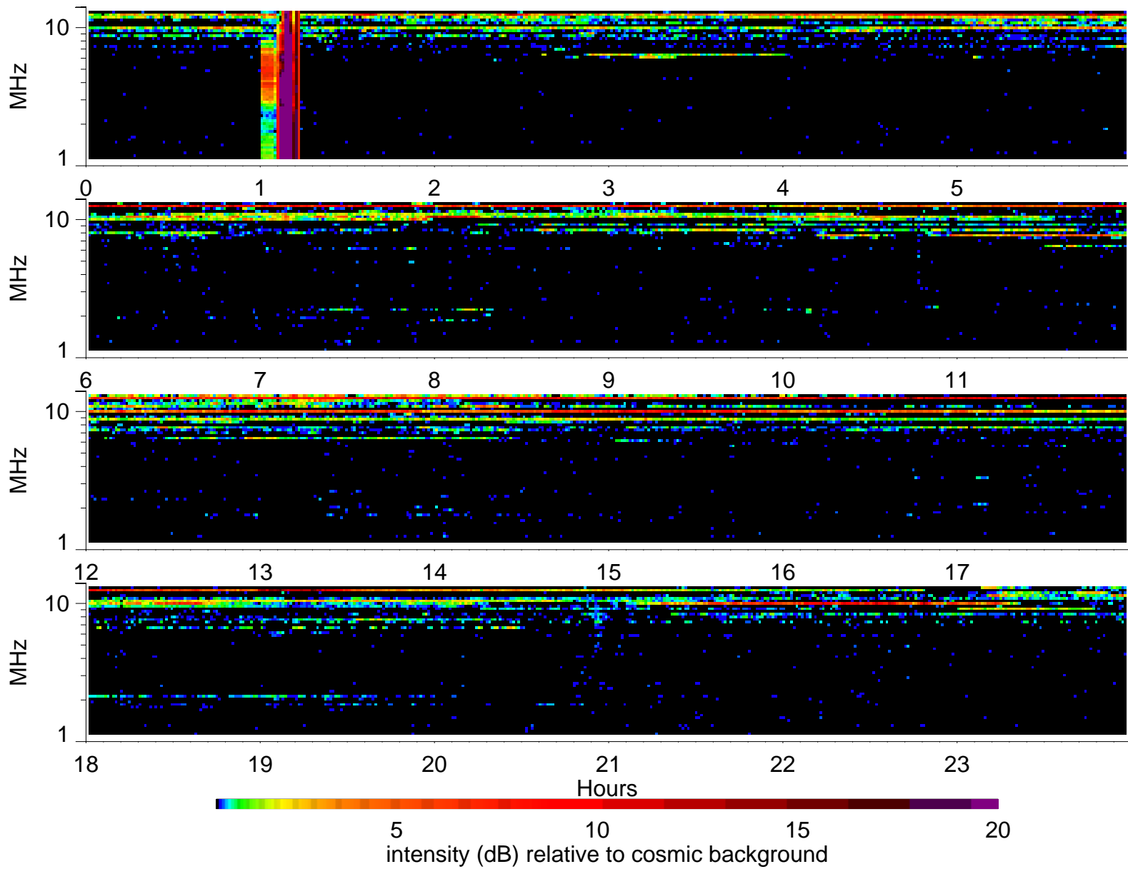
Wind Waves RAD2 receiver: 1995/8/14
