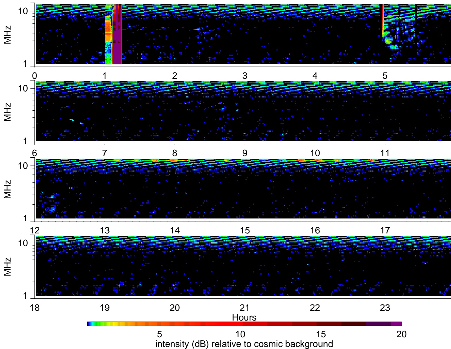
Wind Waves RAD2 receiver: 1995/2/27
