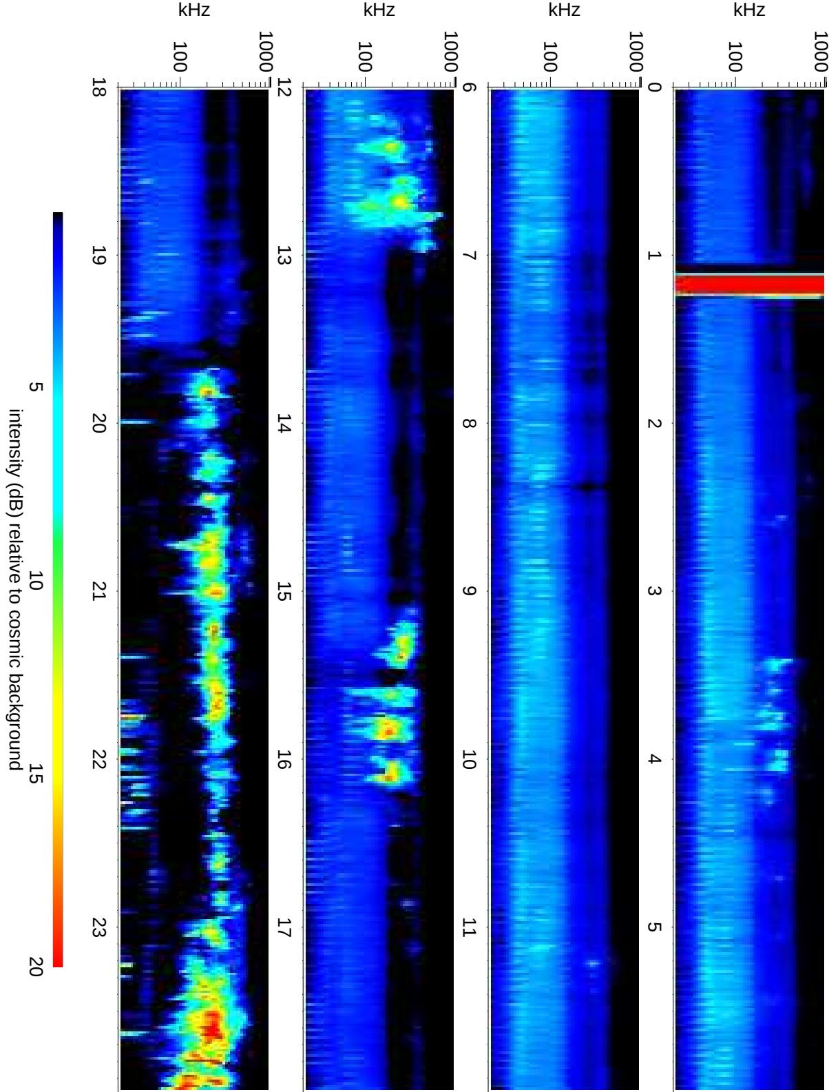
Wind Waves RAD1 receiver: 2017/11/21/24
