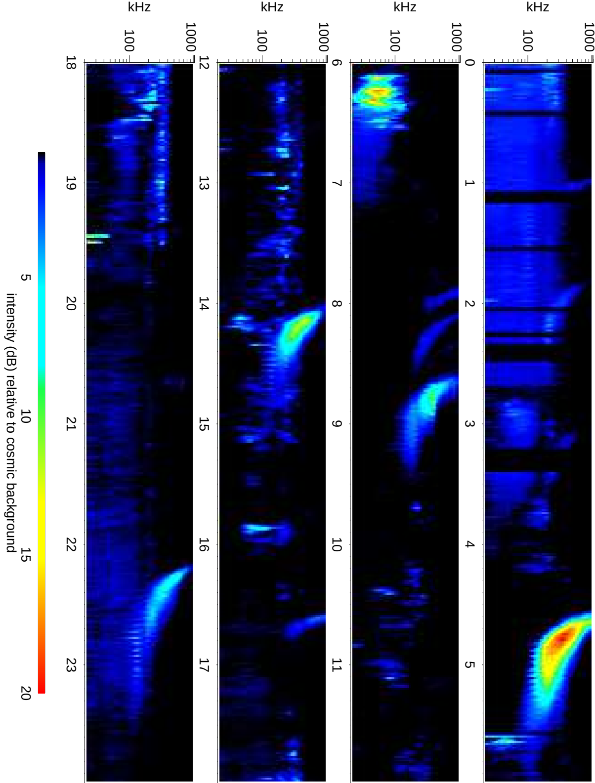
Wind Waves RAD1 receiver: 2015/04/17
