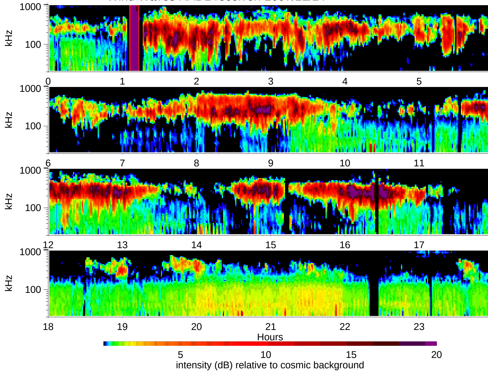
Wind Waves RAD1 receiver: 2007/11/14
