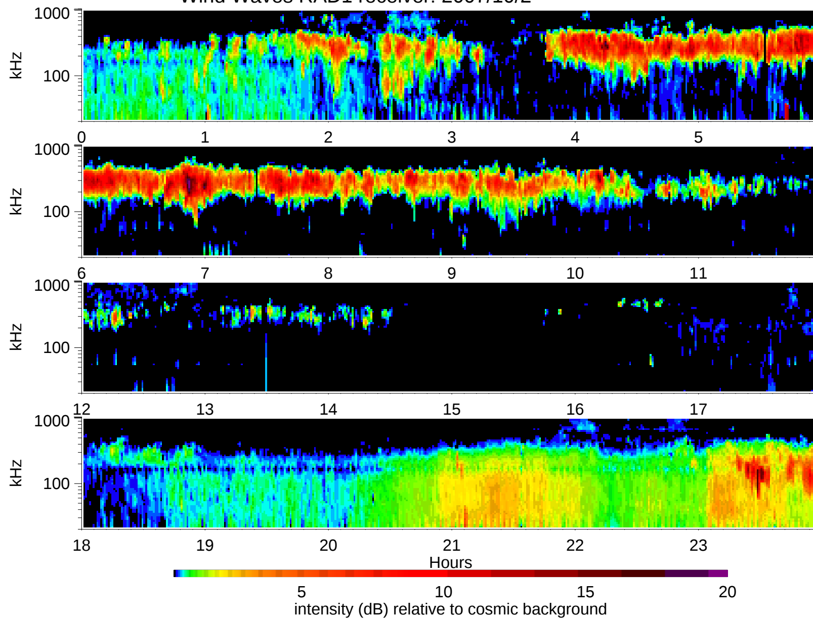
Wind Waves RAD1 receiver: 2007/10/2
