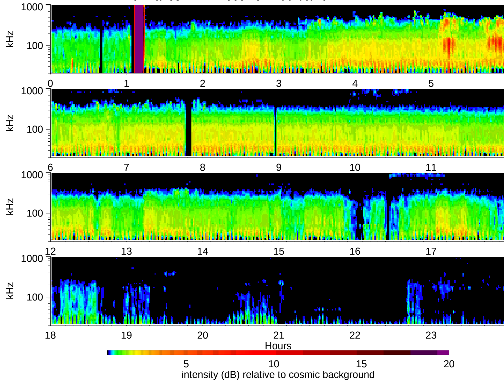
Wind Waves RAD1 receiver: 2007/9/19
