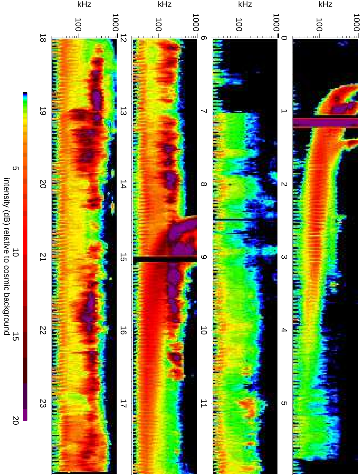
Wind Waves RAD1 receiver: 2007/05/22
