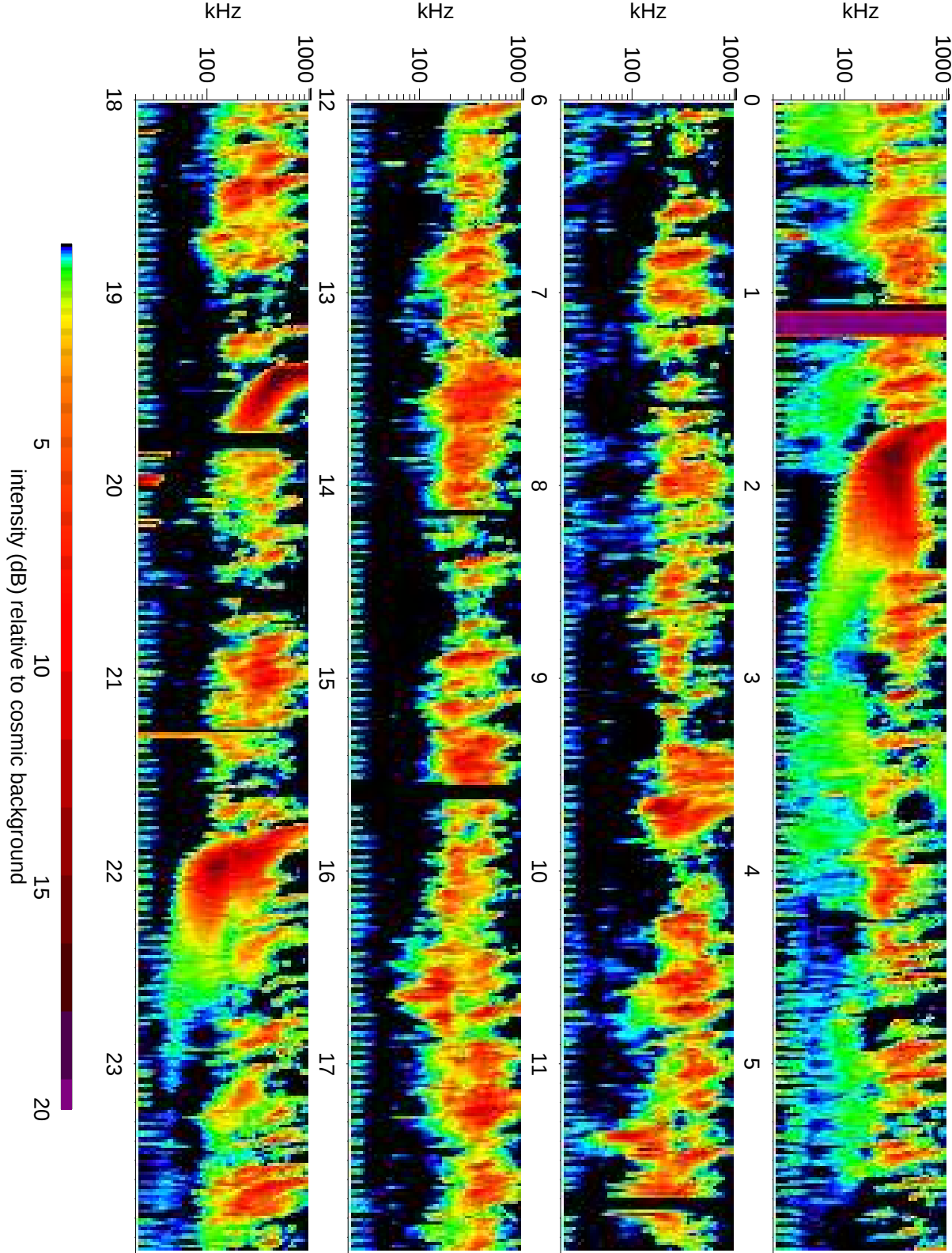
Wind Waves RAD1 receiver: 2007/01/10
