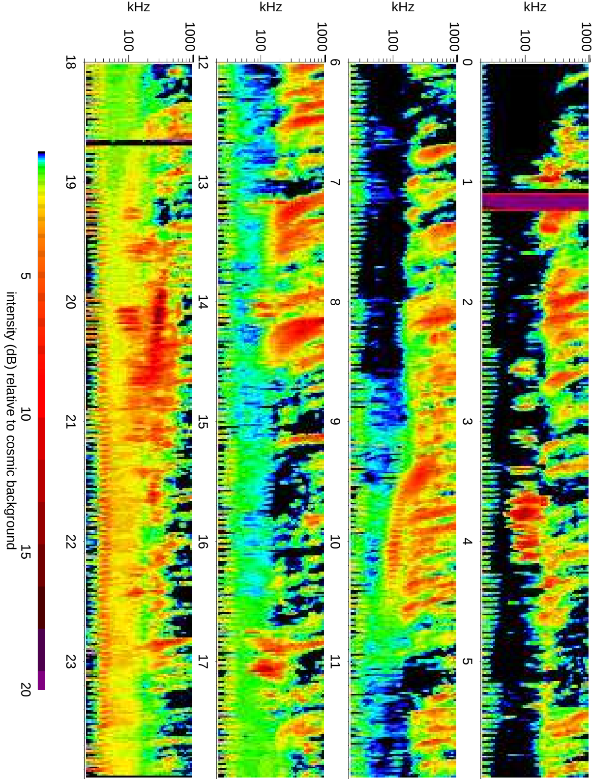
Wind Waves RAD1 receiver: 2007/01/08
