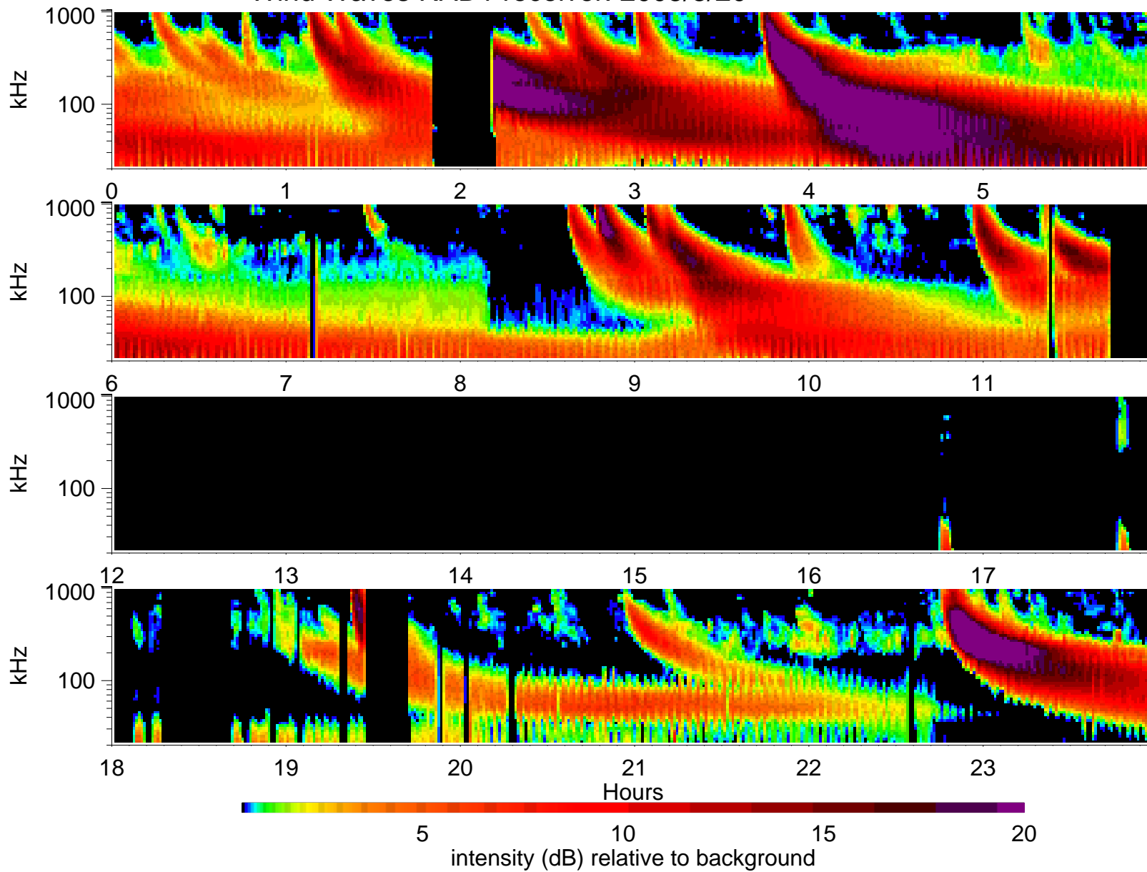
Wind Waves RAD1 receiver: 2005/3/20
