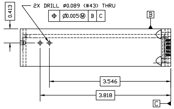
VIEW B-B
