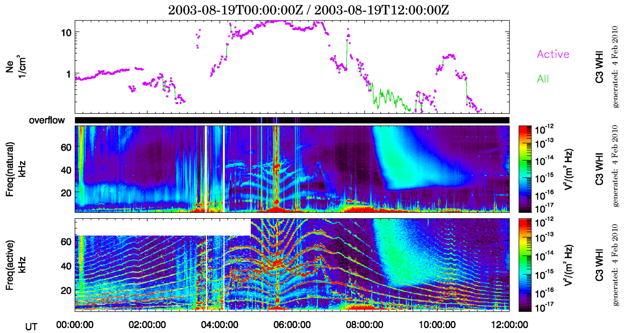
Figure 4: Example of density values and NATURAL and ACTIVE spectrograms (from top to bottom) for C3 on August 19, 2003, corresponding to a plasmasphere crossing. Density values extracted from the ACTIVE WHISPER spectra are plotted as purple points whereas green line represents the density extracted from both ACTIVE and NATURAL measurements. In this interval two methods were used: Max2 for ACTIVE and UpperCutoff for NATURAL.
