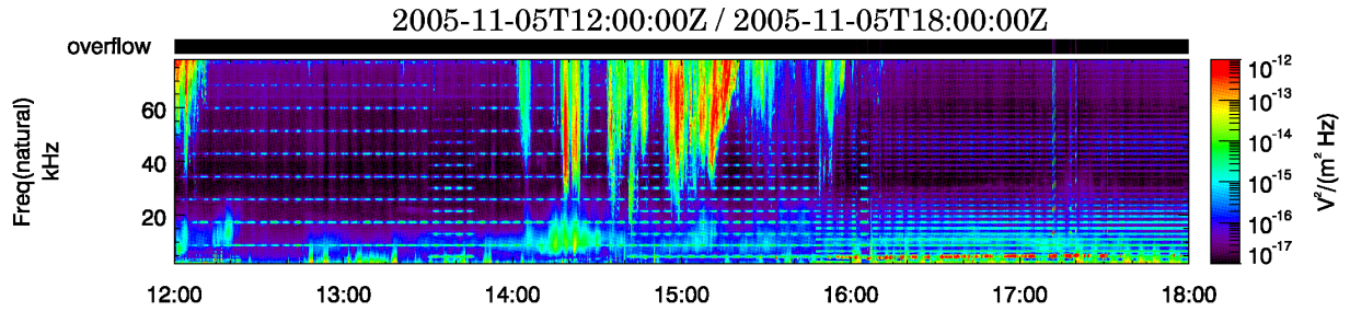
Figure 3: Example of EDI perturbations for C3 on November 05, 2005. EDI interferences appear as horizontal harmonic lines with fundamental frequency depending on the EDI operation mode.
