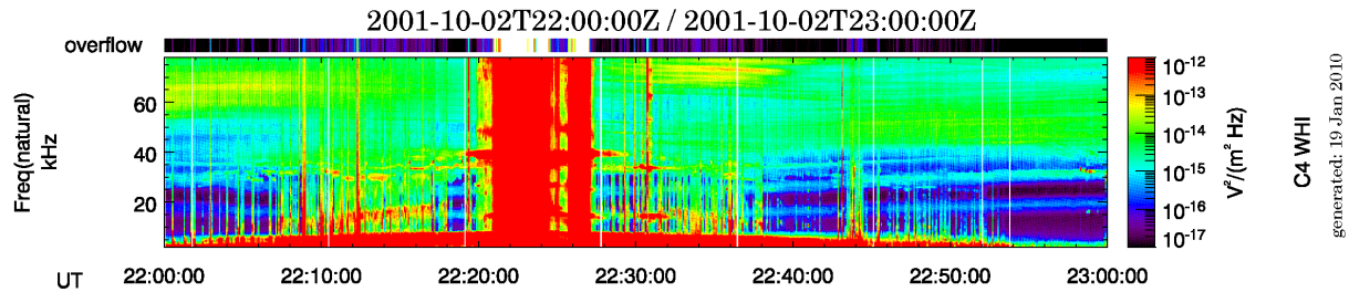
Figure 2: Example of a WHISPER electric spectral power density spectrogram affected by overflows on C4 for October 02, 2001. The upper bar gives the colour-coded overflow rate.
