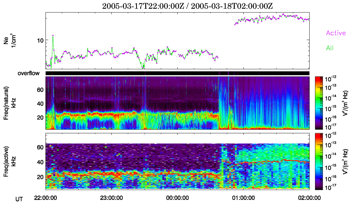
Figure 5: Example of density values and NATURAL and ACTIVE spectrograms (from top to bottom) for C3 on March 17, 2005, corresponding to solar wind/magnetosheath transition. Density values extracted from the ACTIVE WHISPER spectra are plotted as purple points whereas green line represents the density extracted from both ACTIVE and NATURAL measurements. In this interval two methods were used: Max2_EFW for ACTIVE and Proxy_EFW for NATURAL.
