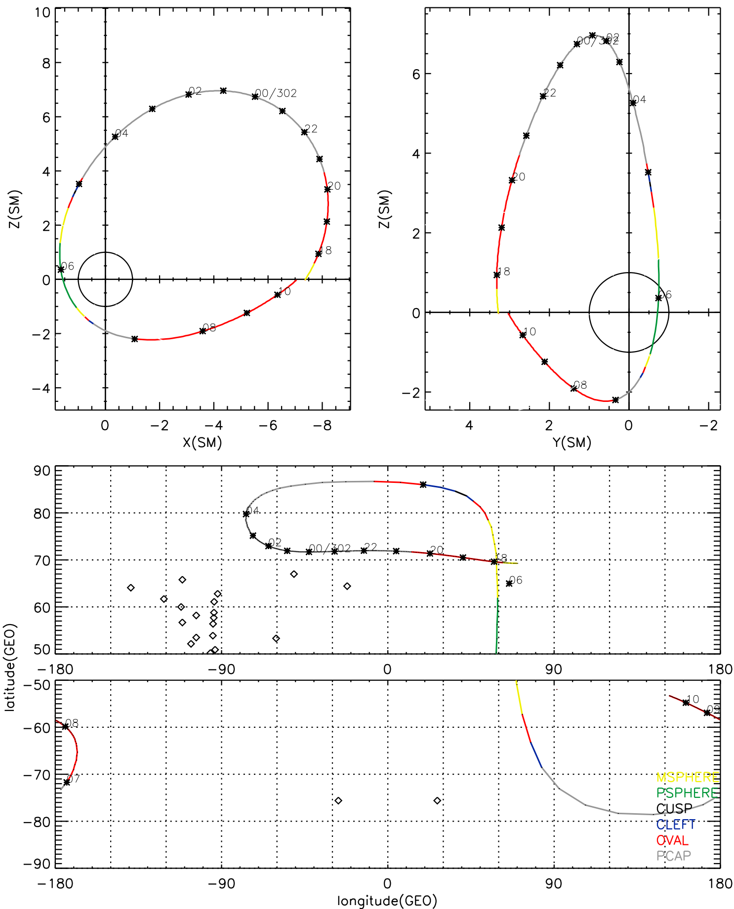
POLAR orbit 2000 301 (10/27) 17:09 UT to 2000 302 (10/28) 10:51 UT
