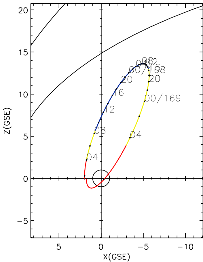
CLUSTER 2 orbit 2024 167 (06/15) 01:41 UT to 2024 169 (06/17) 07:51 UT
