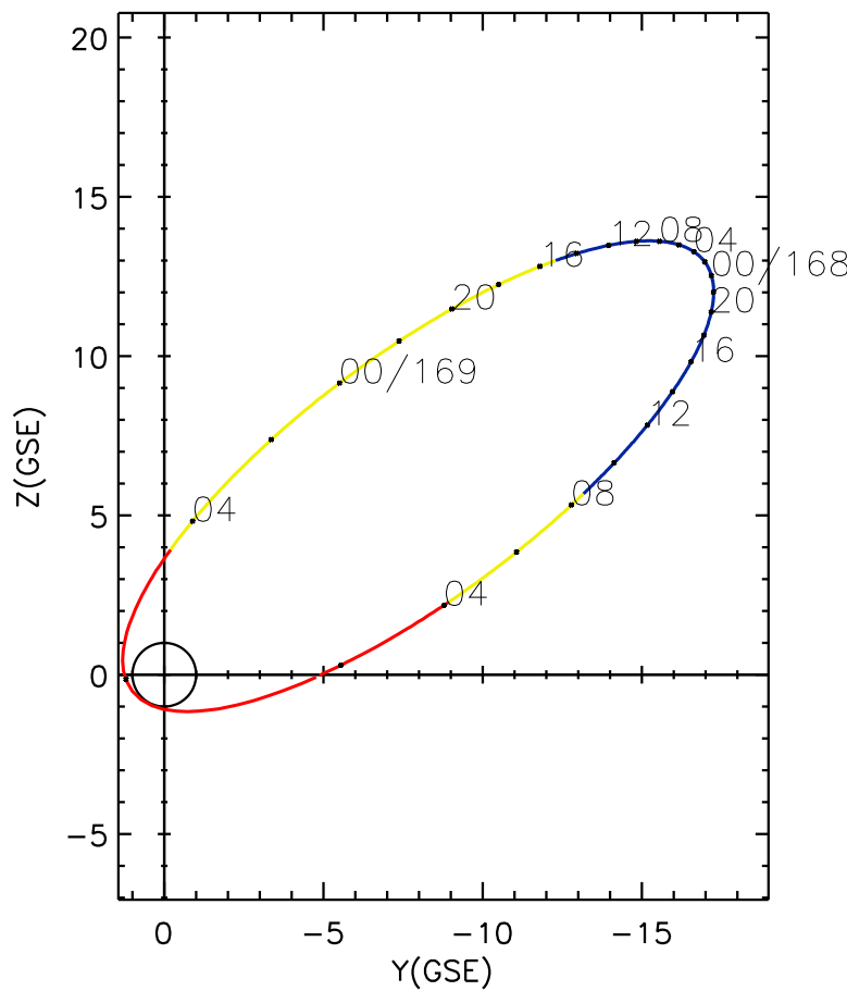
CLUSTER 2 orbit 2024 167 (06/15) 01:41 UT to 2024 169 (06/17) 07:51 UT
