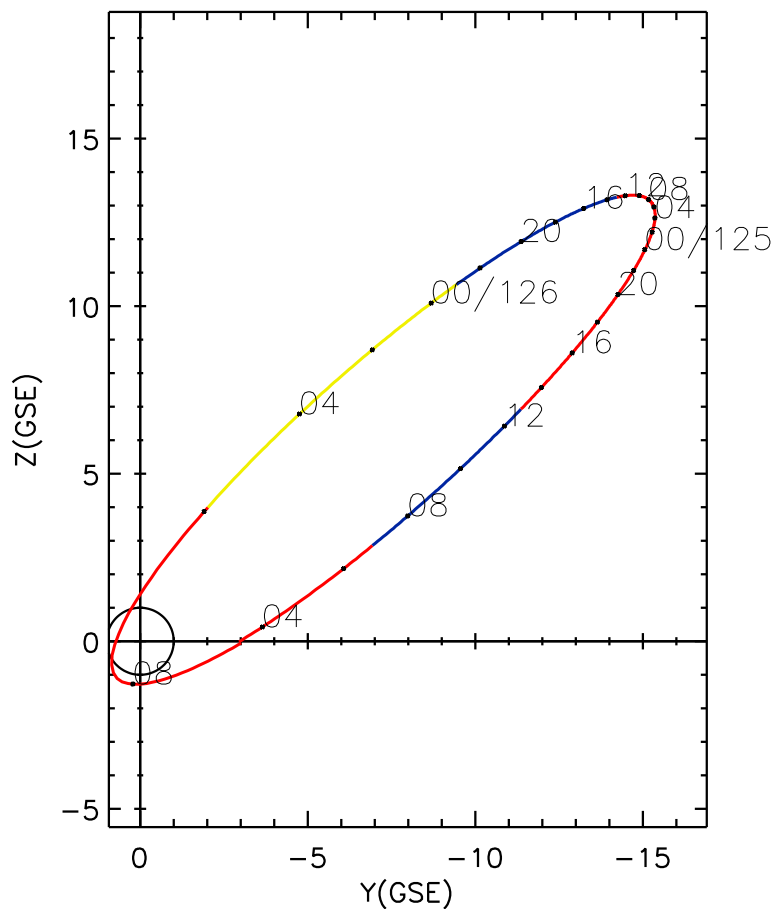
CLUSTER 2 orbit 2024 124 (05/03) 03:31 UT to 2024 126 (05/05) 09:41 UT
