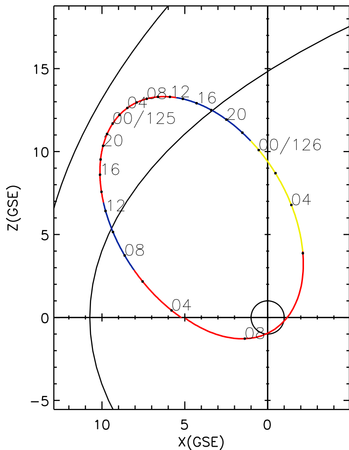
CLUSTER 2 orbit 2024 124 (05/03) 03:31 UT to 2024 126 (05/05) 09:41 UT
