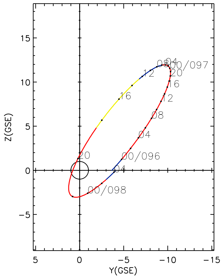
CLUSTER 2 orbit 2023 095 (04/05) 22:01 UT to 2023 098 (04/08) 04:16 UT
