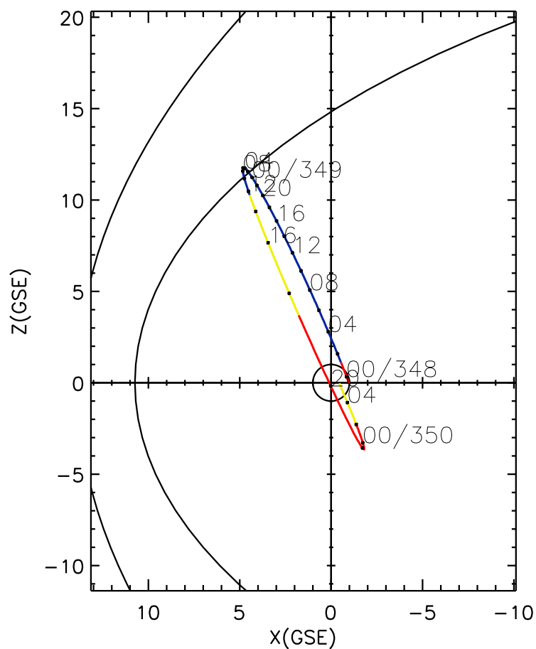
CLUSTER 2 orbit 2022 347 (12/13) 23:26 UT to 2022 350 (12/16) 05:41 UT
