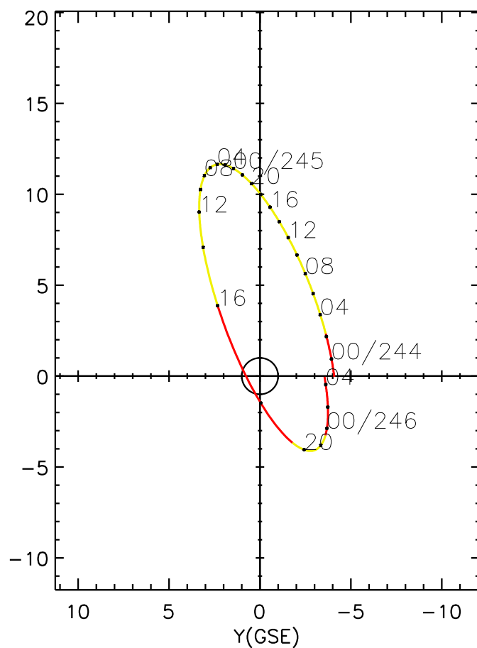
CLUSTER 2 orbit 2022 243 (08/31) 22:26 UT to 2022 246 (09/03) 04:41 UT
