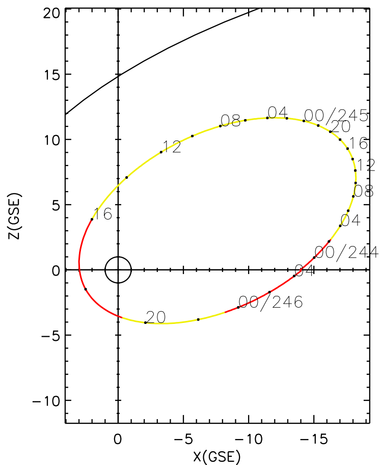
CLUSTER 2 orbit 2022 243 (08/31) 22:26 UT to 2022 246 (09/03) 04:41 UT
