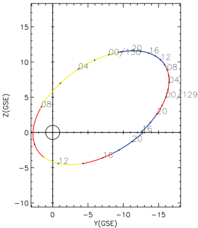
CLUSTER 2 orbit 2022 128 (05/08) 15:46 UT to 2022 130 (05/10) 22:01 UT
