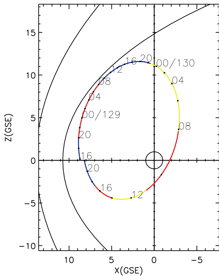
CLUSTER 2 orbit 2022 128 (05/08) 15:46 UT to 2022 130 (05/10) 22:01 UT
