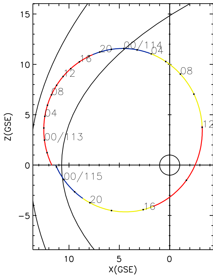
CLUSTER 2 orbit 2022 112 (04/22) 20:01 UT to 2022 115 (04/25) 02:16 UT
