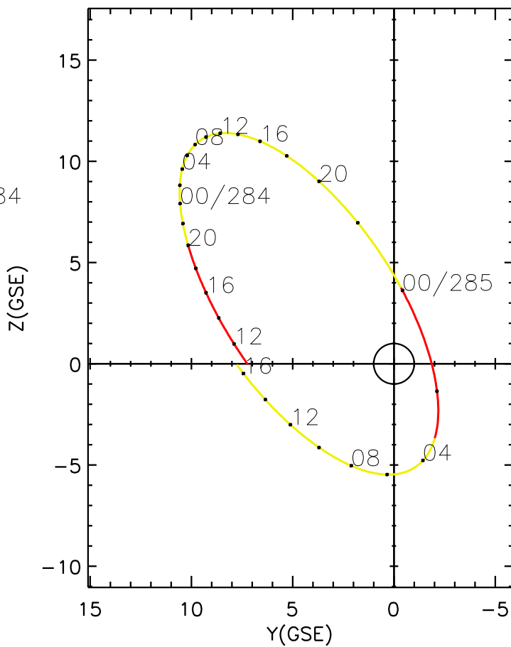
CLUSTER 2 orbit 2021 283 (10/10) 10:26 UT to 2021 285 (10/12) 16:41 UT
