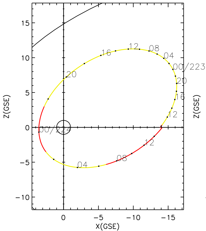
CLUSTER 2 orbit 2021 222 (08/10) 09:41 UT to 2021 224 (08/12) 15:56 UT
