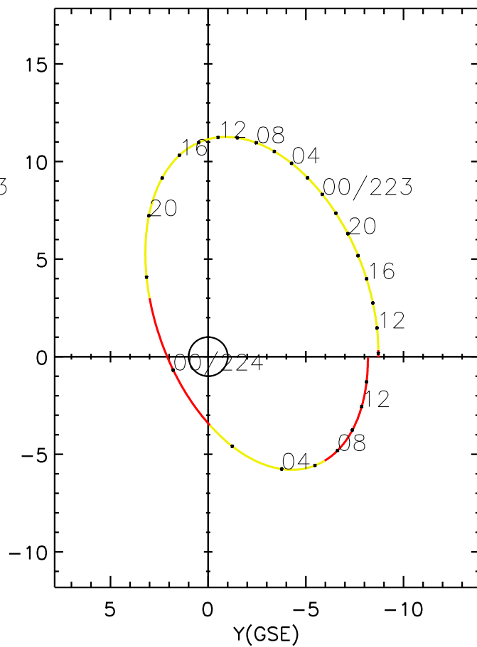
CLUSTER 2 orbit 2021 222 (08/10) 09:41 UT to 2021 224 (08/12) 15:56 UT
