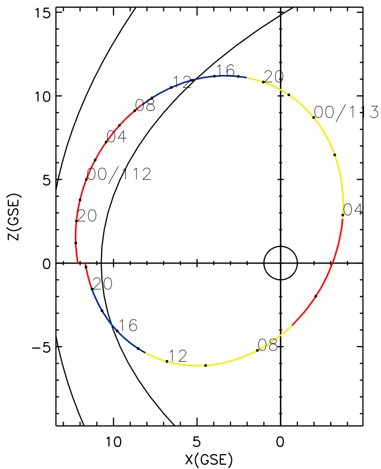
CLUSTER 2 orbit 2021 111 (04/21) 16:06 UT to 2021 113 (04/23) 22:21 UT
