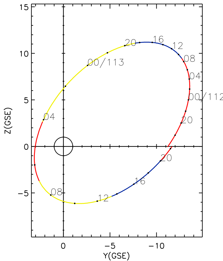
CLUSTER 2 orbit 2021 111 (04/21) 16:06 UT to 2021 113 (04/23) 22:21 UT
