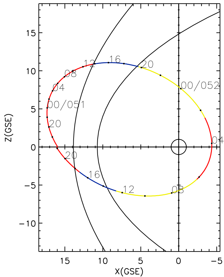
CLUSTER 2 orbit 2021 050 (02/19) 16:01 UT to 2021 052 (02/21) 22:16 UT
