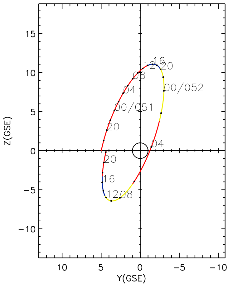
CLUSTER 2 orbit 2021 050 (02/19) 16:01 UT to 2021 052 (02/21) 22:16 UT
