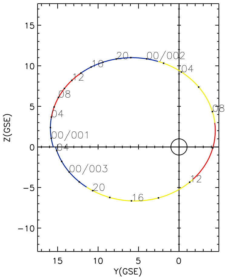
CLUSTER 2 orbit 2020 366 (12/31) 22:21 UT to 2021 003 (01/03) 04:36 UT
