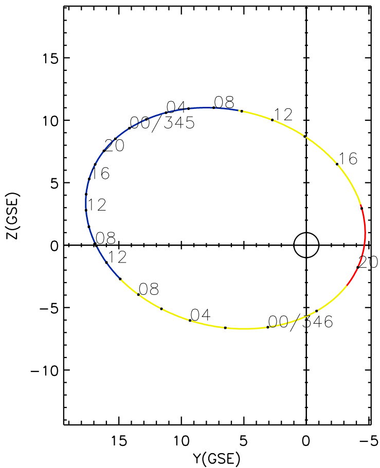
CLUSTER 2 orbit 2020 344 (12/09) 07:46 UT to 2020 346 (12/11) 14:01 UT
