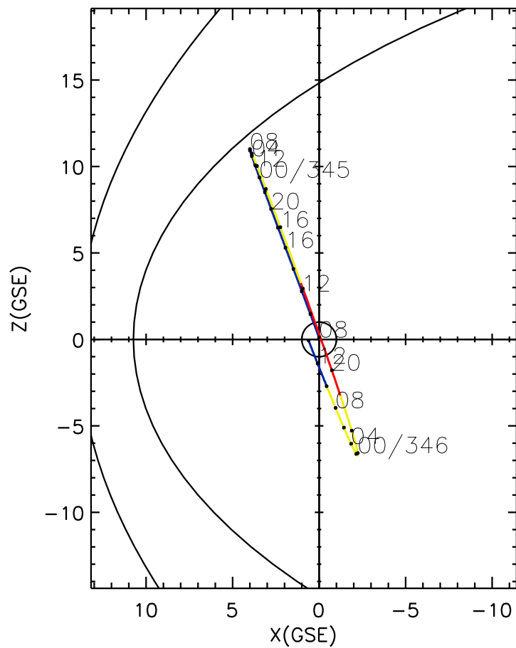
CLUSTER 2 orbit 2020 344 (12/09) 07:46 UT to 2020 346 (12/11) 14:01 UT
