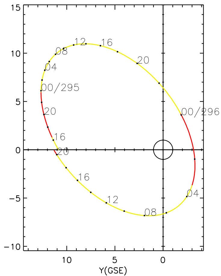
CLUSTER 2 orbit 2020 294 (10/20) 14:31 UT to 2020 296 (10/22) 20:41 UT
