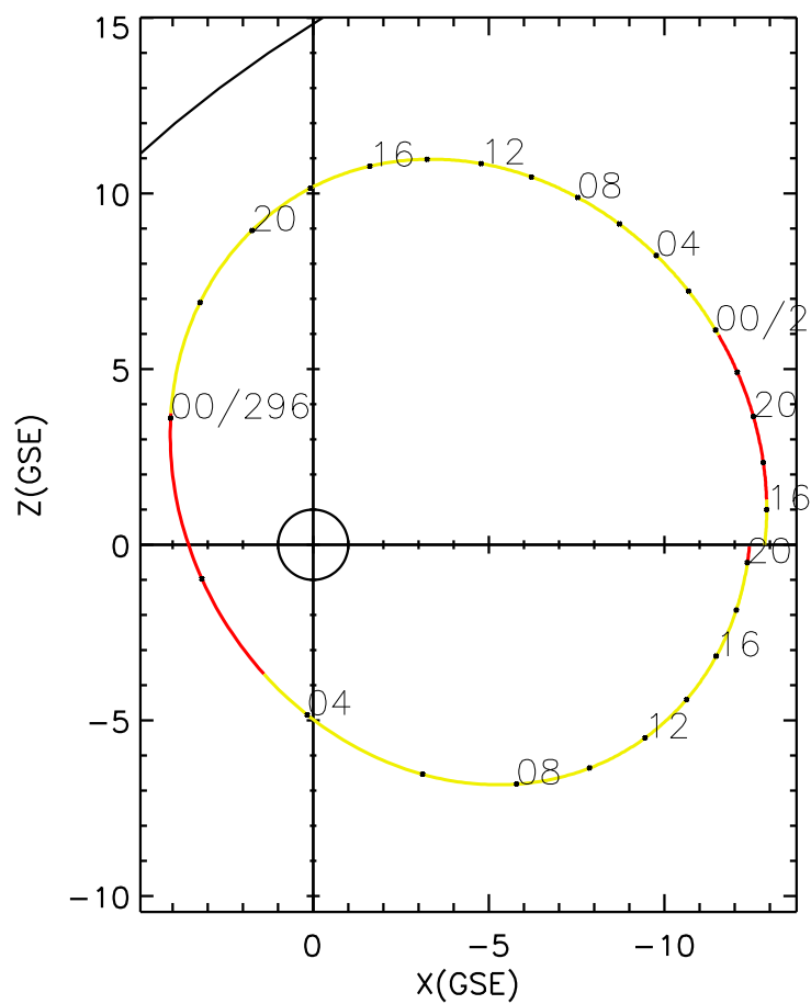
CLUSTER 2 orbit 2020 294 (10/20) 14:31 UT to 2020 296 (10/22) 20:41 UT
