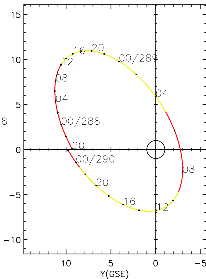
CLUSTER 2 orbit 2020 287 (10/13) 19:51 UT to 2020 290 (10/16) 02:01 UT
