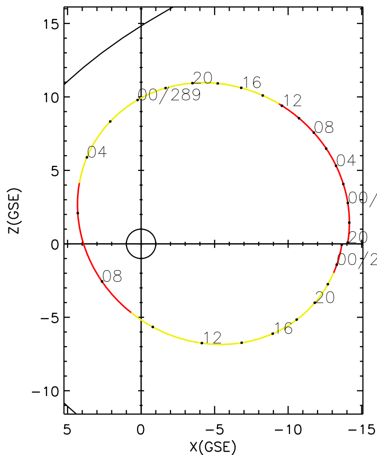
CLUSTER 2 orbit 2020 287 (10/13) 19:51 UT to 2020 290 (10/16) 02:01 UT
