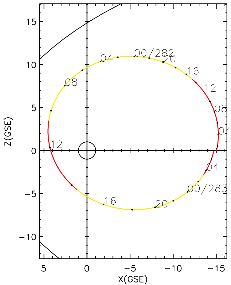
CLUSTER 2 orbit 2020 281 (10/07) 01:11 UT to 2020 283 (10/09) 07:26 UT
