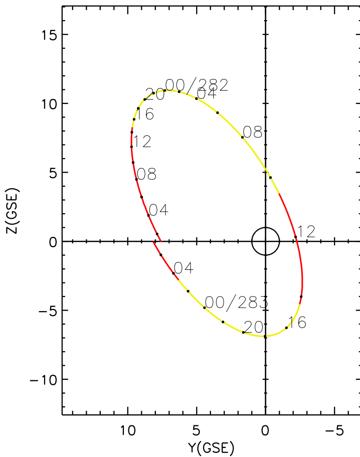
CLUSTER 2 orbit 2020 281 (10/07) 01:11 UT to 2020 283 (10/09) 07:26 UT
